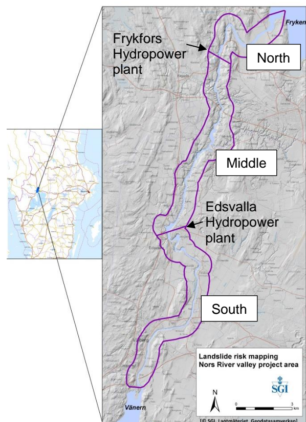
Figure 1. River Norsälven from Lake Lower Fryken to Lake Vänern. The figure displays the area in hill shaded topography and shows the investigated area as part of the Landslide risk analysis. The stretch is divided into three parts separated by two hydropower plants. © SGI, Lantmäteriet, Geodatasamverkan.
